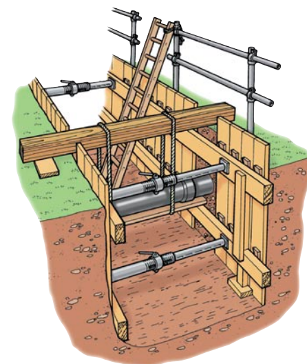
Figure 44 An excavation supported by timbering and props with guard rails (omitted from left-hand side for clarity) to prevent falls. Extended poling boards act as toe boards, safe access is provided by a tied ladder and exposed services are supported
