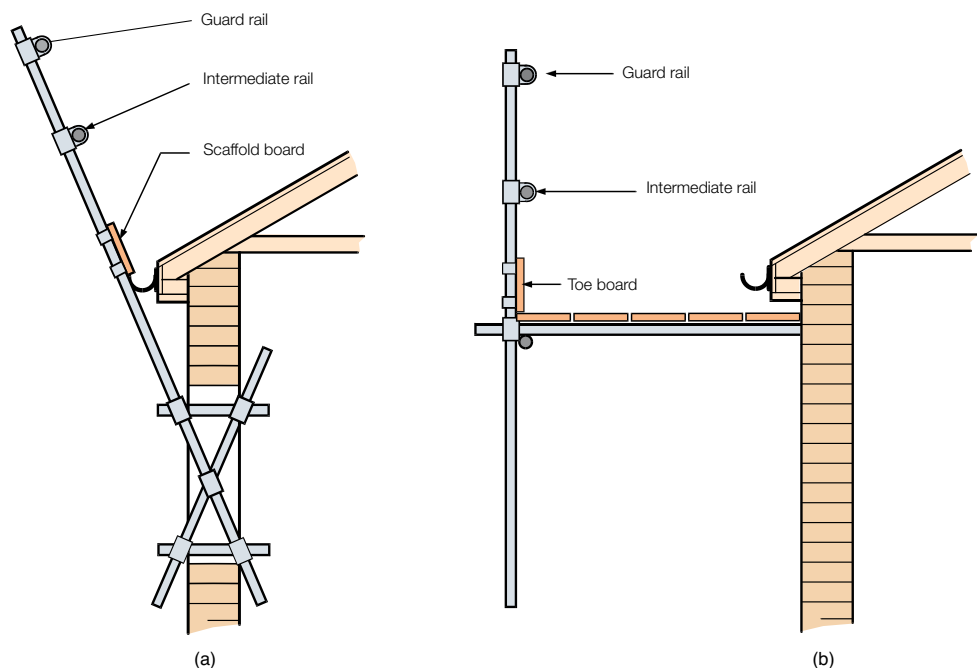
Figure 23 Typical sloping-roof edge protection
